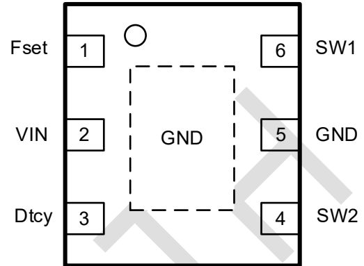
DFN2×2-6
