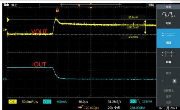
图 3 Load Transient ( V_{IN}=V_{OUT}+1V , I_{OUT}=0mA-500mA )
