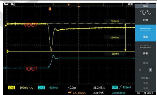
图 4 Load Transient ( V_{IN}=V_{OUT}+1V , I_{OUT}=500mA-0mA )
