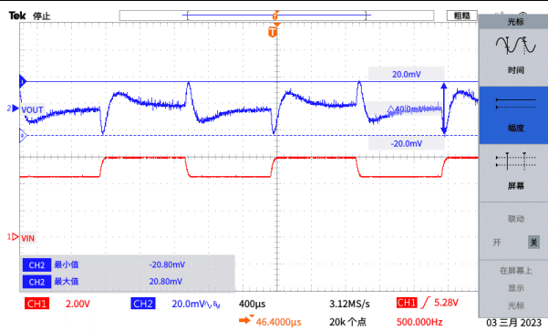
图 1 Line Transient ( V_{IN} =from V_{OUT}+1V to 6V to V_{OUT}+1V , I_{OUT}=50mA )
