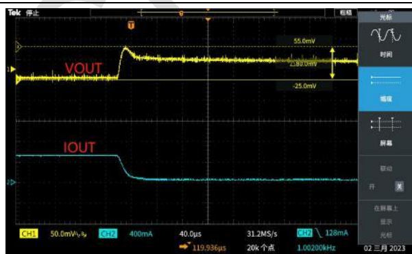
图 5 Load Transient ( V_{IN}=V_{OUT}+1V , I_{OUT}=50mA-500mA )
