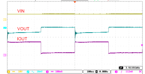
图 4 Load Transient ( V_{IN} =7V, I_{OUT} =1mA-150mA-1mA)
