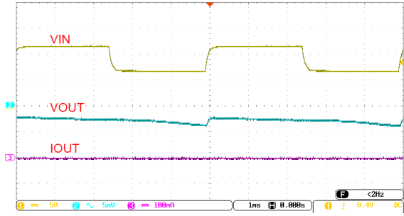
图 1 Line Transient ( V_{IN} =from 6V to 12V to V_{OUT}+1V I_{OUT} =0mA)
